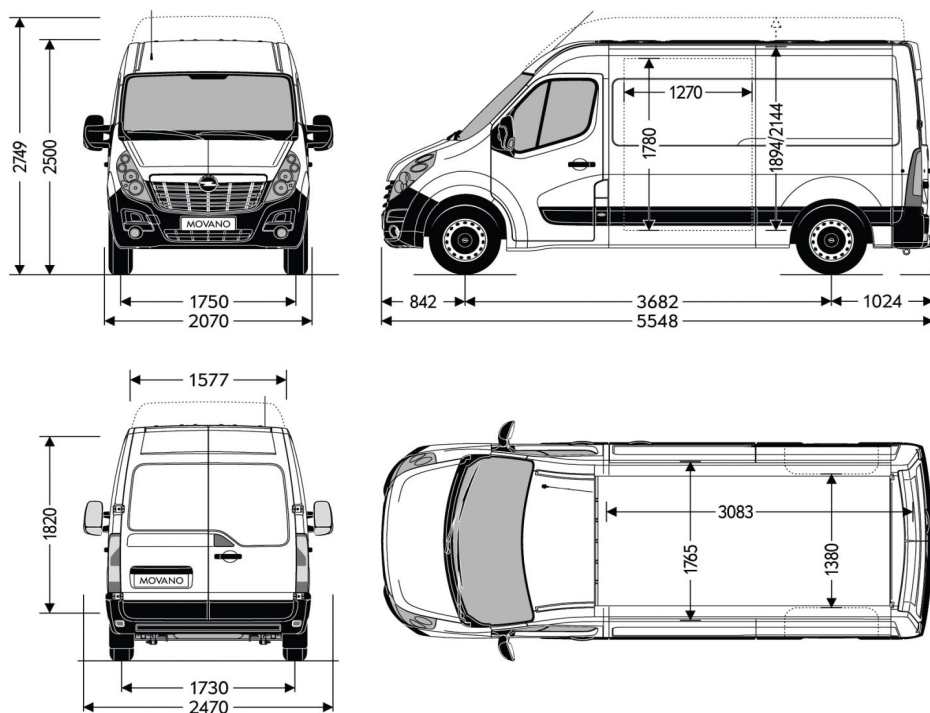
Opel Movano Van FWD L2H2-H3
