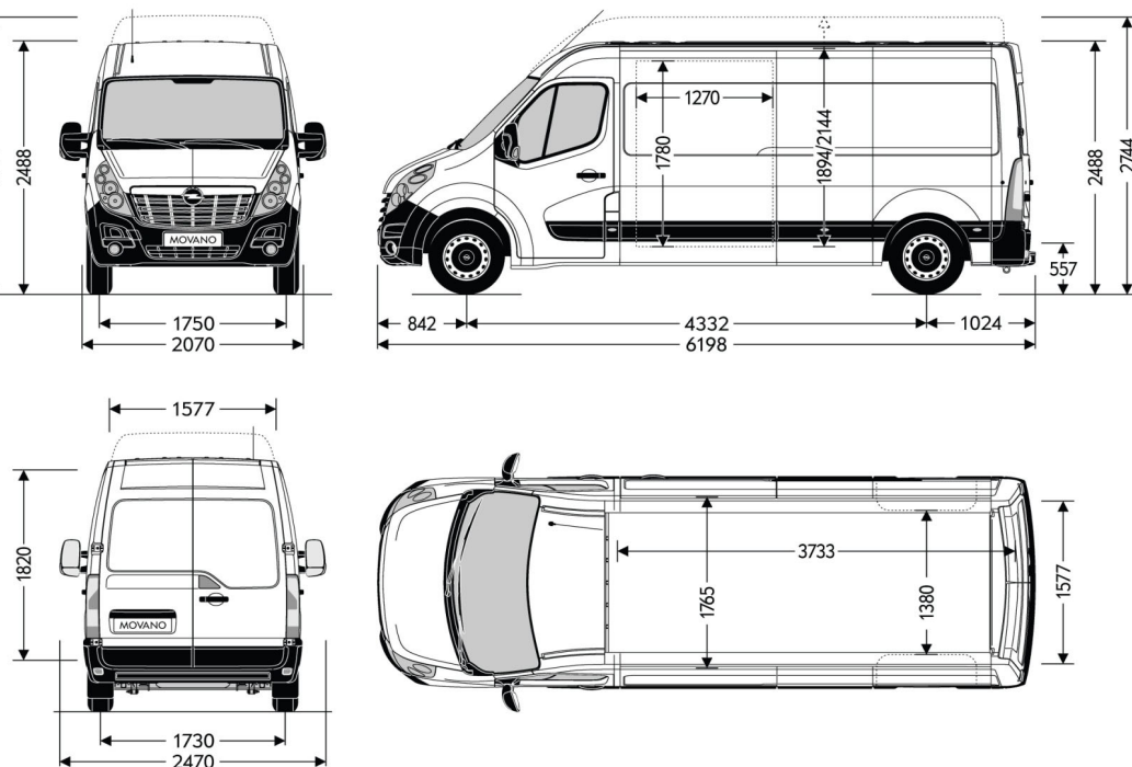
Opel Movano Van FWD L3H2-H3
