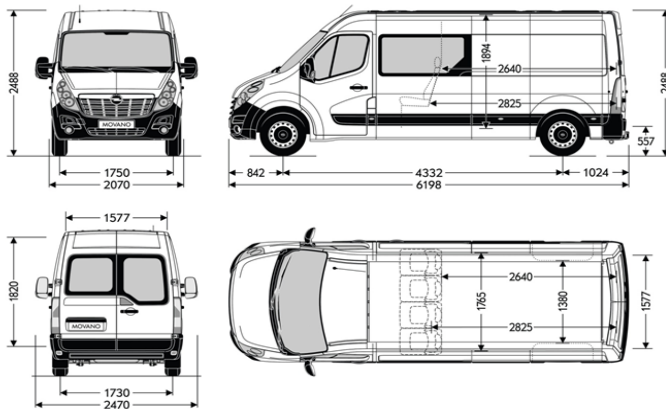
Opel Movano Crew Van FWD L3H2
